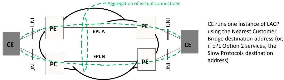
Figure 10 – Link Aggregation of EPL Services
